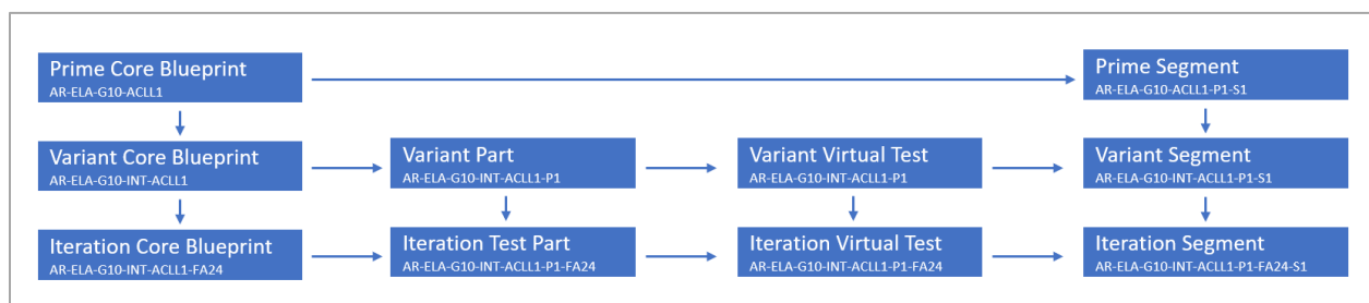
Figure 138. Hierarchy of Blueprint Relationships
